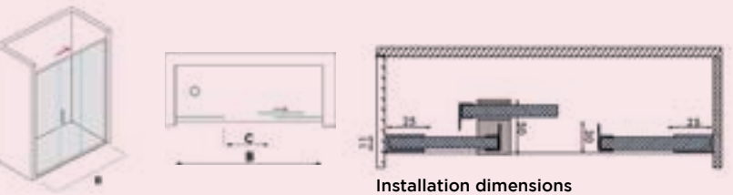
Installation dimensions
