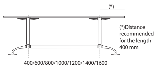
Join bar (measure between axis)
