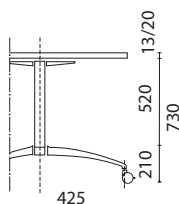
Long leg with castors
