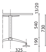
Long leg with glides
