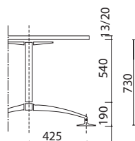
Long leg with glides
