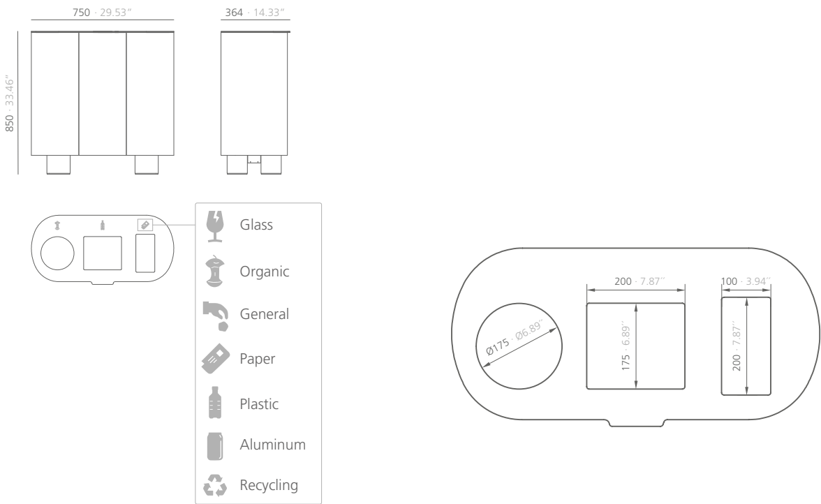
Croma paper bin L / Dimensions: 750x850x364 mm Lacquered structure and legs
