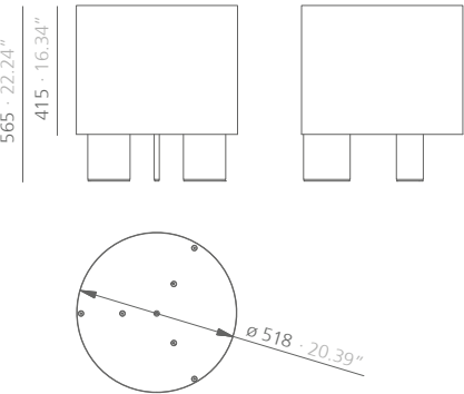
Croma planter L / Dimensions: 518x565x518 mm Lacquered structure and legs
