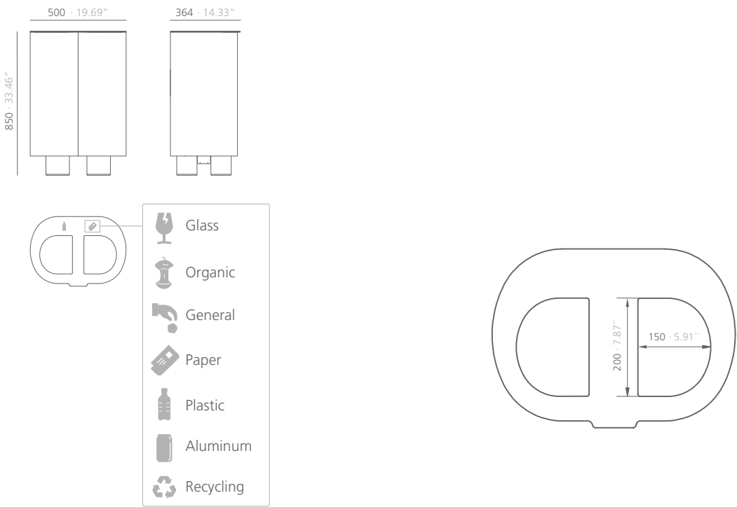
Croma paper bin M / Dimensions: 500x850x364 mm Lacquered structure and legs
