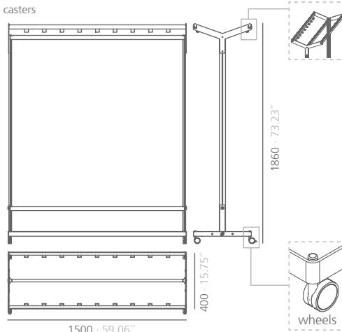
INLD15RD casters
