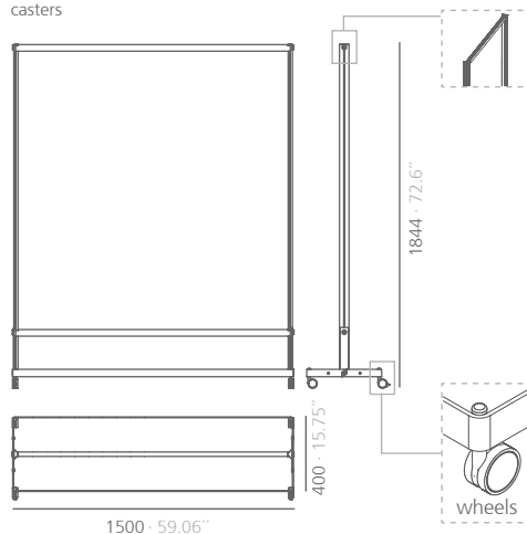
INLD15RD casters
